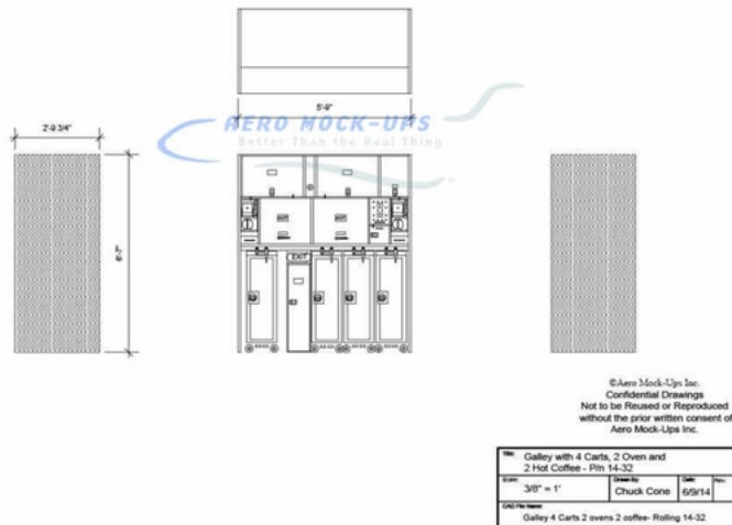
14-32 Galley, Rolling, 4 Carts, 2 Ovens, 2 Coffee
